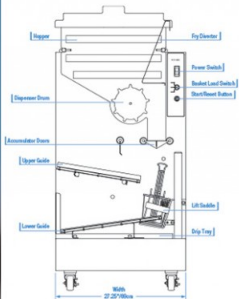
FRONT VIEW
